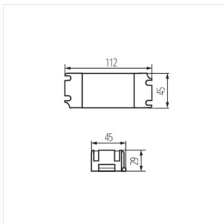
DRIVE LED 0-15W 12VDC
